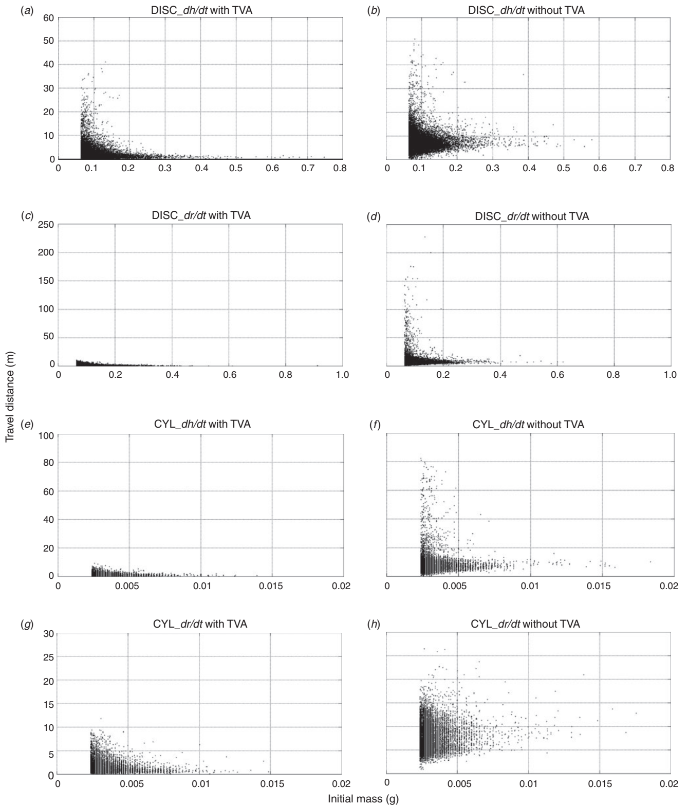
Fig. 7. Travel distance v. initial mass of various firebrand models in surface fire simulation with 6-m s -1 wind at the mid-flame height: (a) DISC_dh/dt with terminal velocity approximation (TVA); (b) DISC_dh/dt without TVA; (c) DISC_dr/dt with TVA; (d) DISC_dr/dt without TVA; (e) CYL_dh/dt with TVA; (f) CYL_dh/dt without TVA; (g) CYL_dr/dt with TVA; and (h) CYL_dr/dt without TVA.
