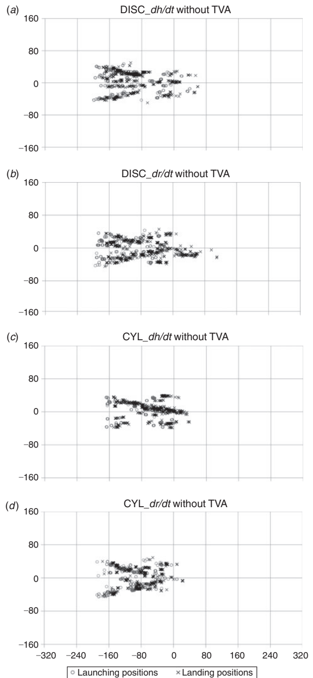
Fig. 8. Launching positions (grey circles) and landing positions (black crosses) of 500 firebrands with the furthest travel distance for various models without terminal velocity assumption in surface fire simulations with a 6\text{-m s}^{-1} wind at mid-flame height on the 640 \times 320\text{-m} domain: (a) DISC_{dh/dt} without TVA; (b) DISC_{dr/dt} without TVA; (c) CYL_{dh/dt} without TVA; and (d) CYL_{dr/dt} without TVA.
